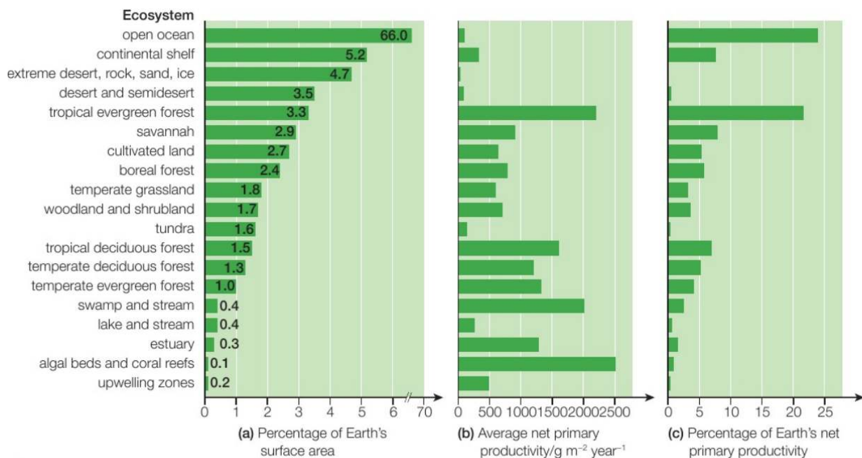
fig C Different ecosystems contribute different amounts to the NPP of the Earth.
